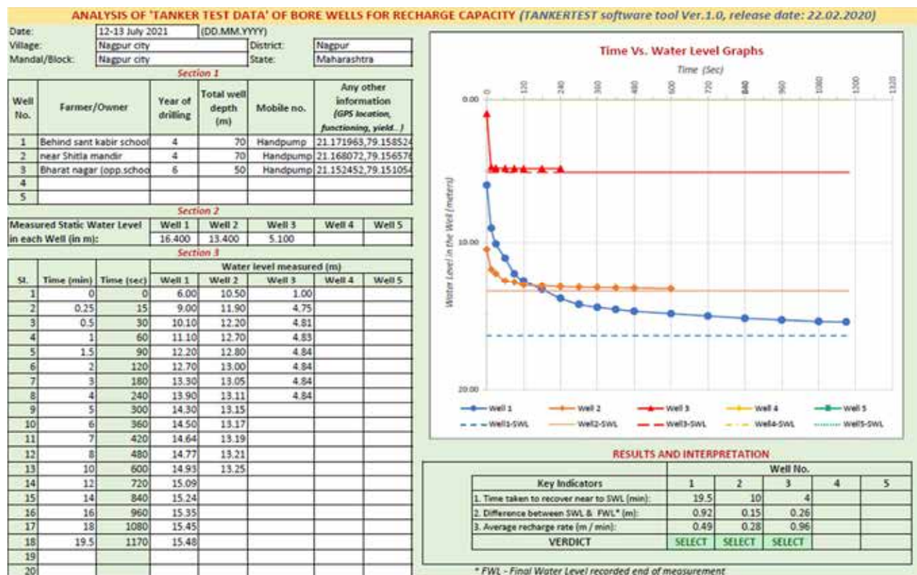
Borewell Recharge Test Source - (ICLEI & Pandey, n.d.)
