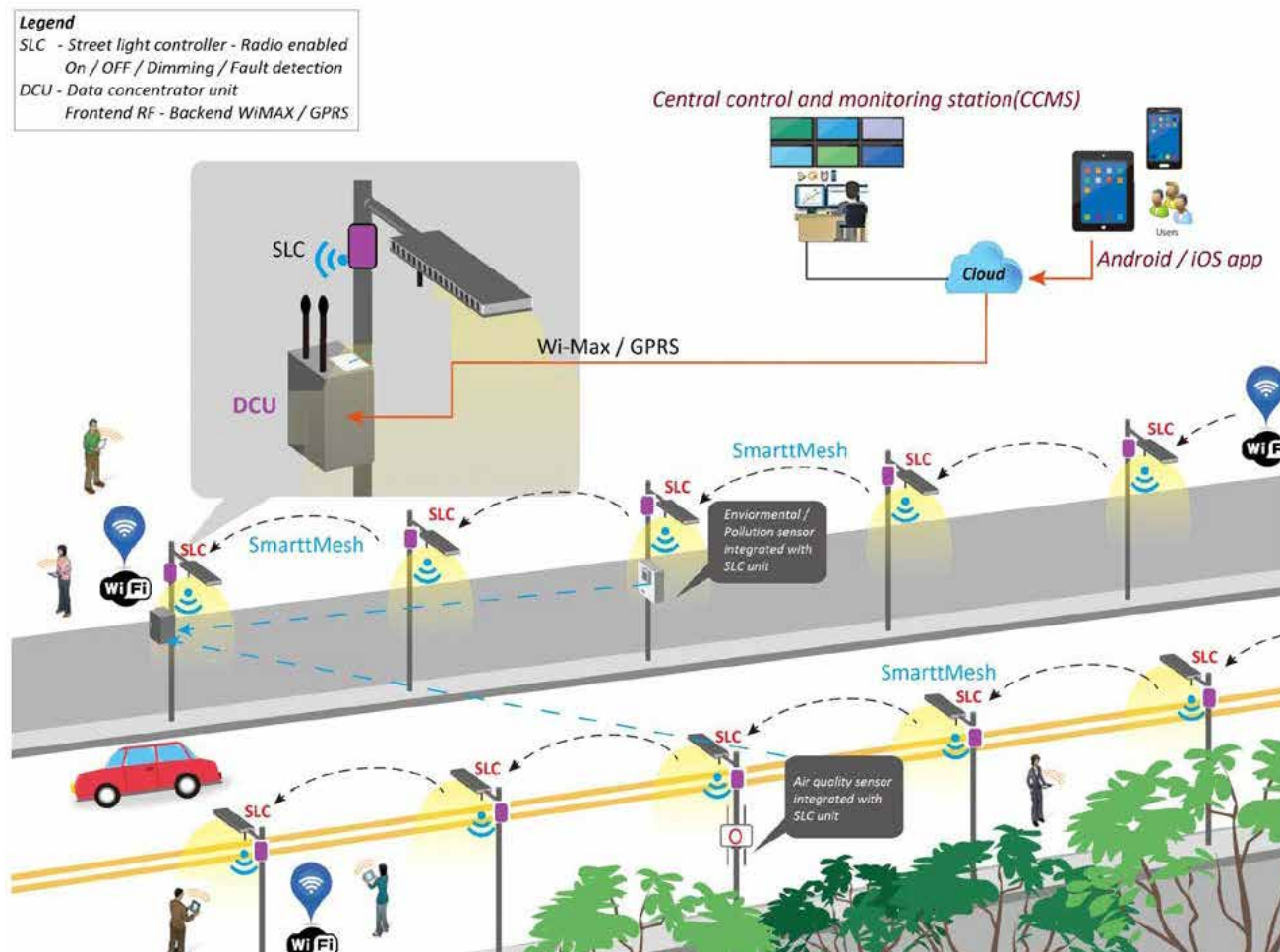
Figure 4: Representation of Smart Streetlight System
