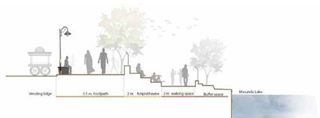
Figure 8: Section through Boating junction, Source: Author
