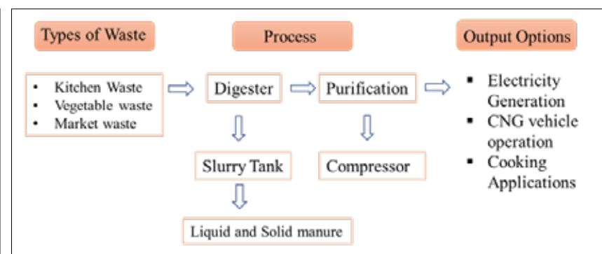
Figure 4: Process flow of the Choithram Mandi Plant
