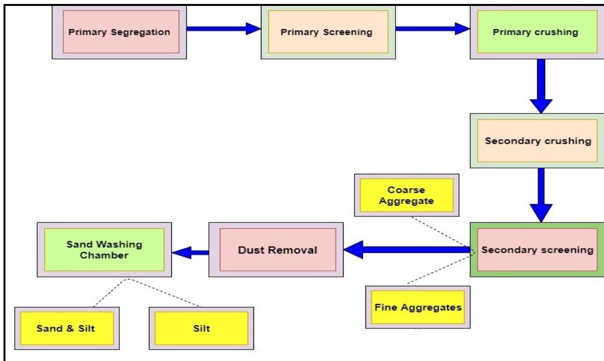
Figure 25: Process layout for Wet Processing of C&D waste
