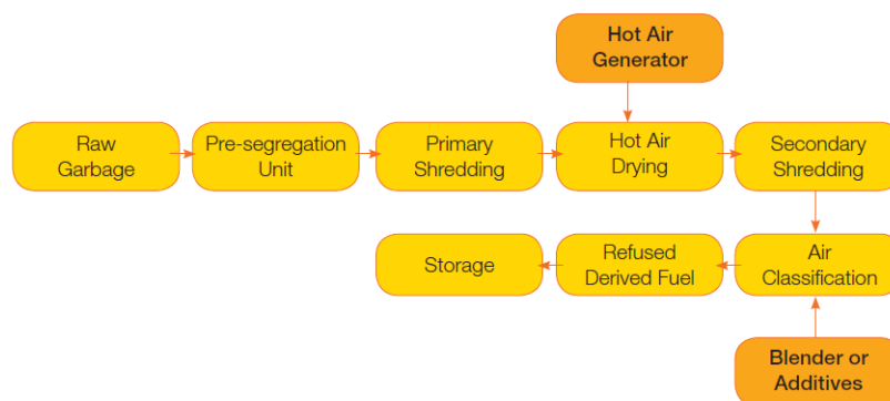
Figure: RDF Generation
