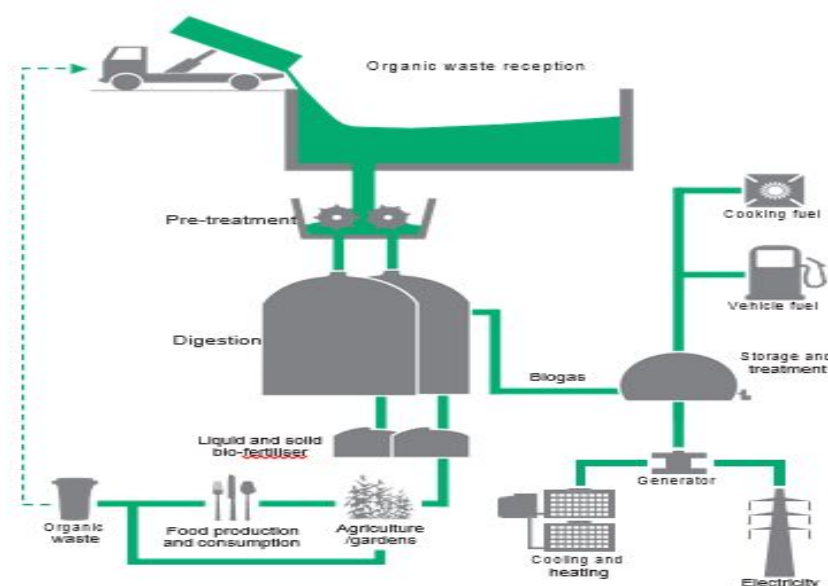
Figure 14: Typical Circularity in Biomethanation Process Flow
