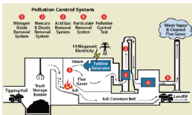
Figure: Waste Incineration
