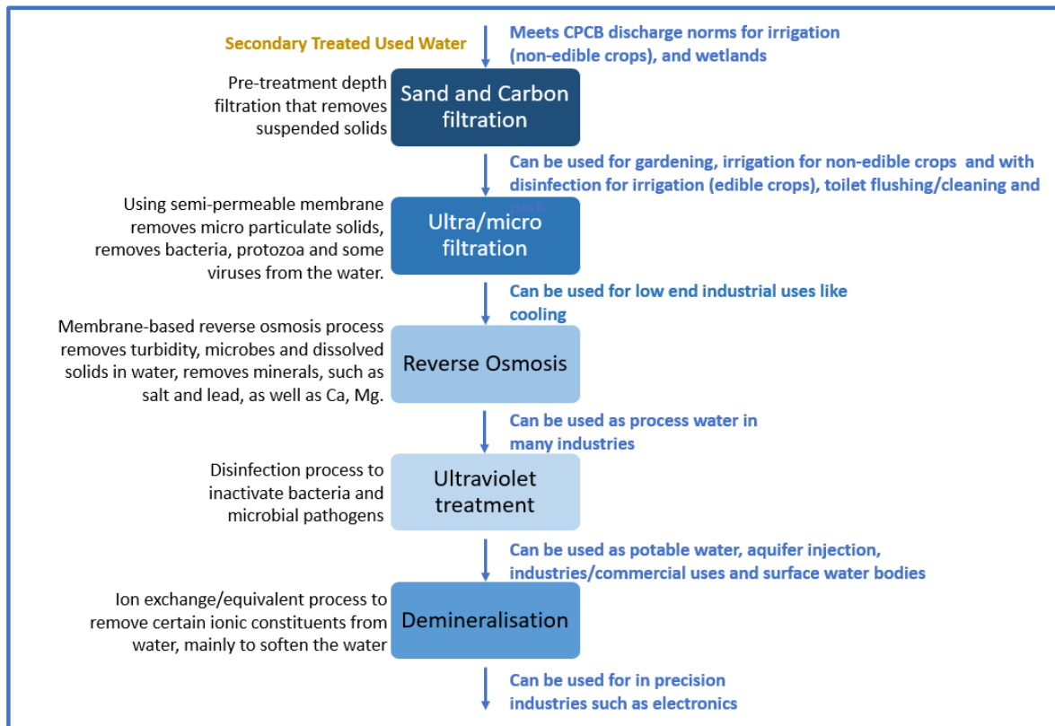
Figure 29: Incremental Technology interventions to achieve End Use Water Quality Standards (Source: Draft National Policy on the Safe Reuse of Treated Wastewater, India- EU Partnership)
