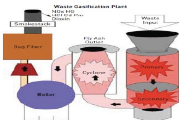
Figure: Gasification
