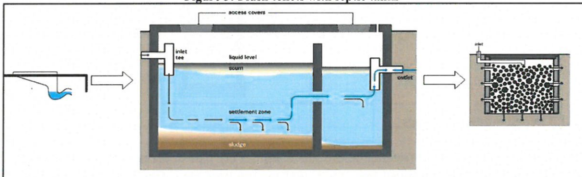
Figure 3: Flush toilets with septic tanks
