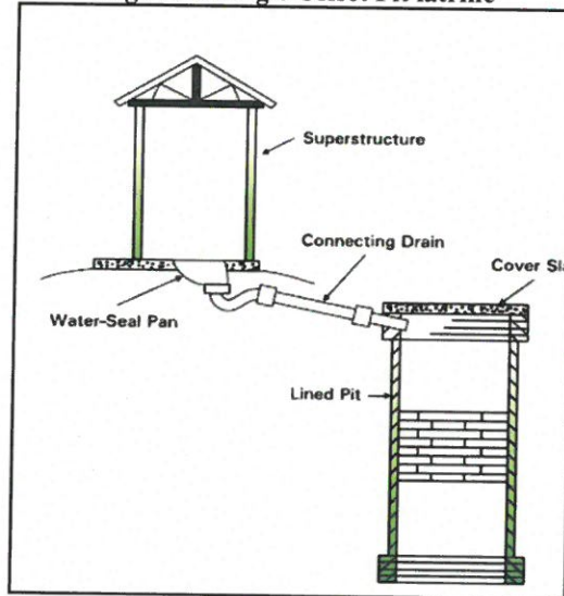
Figure 1: Single Offset Pit latrine
